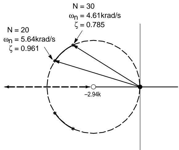
Figure 12. Root Locus Variation
